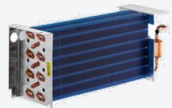
Evaporator Coil
